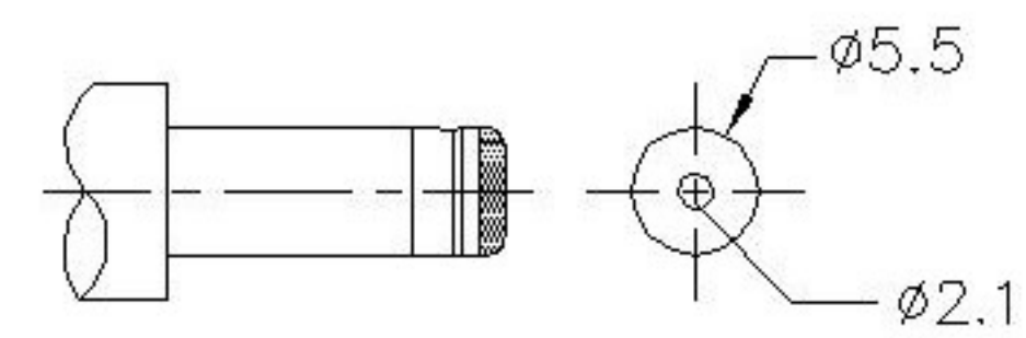
MATING PLUG Jack Insertion Depth: 9.15 mm
