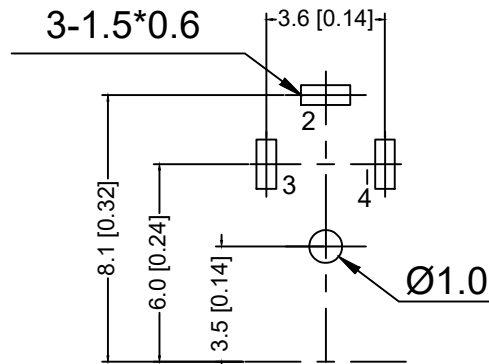
PCB HOLES(TOP VIEW) GENERAL TOLERANCE:0.1MM
