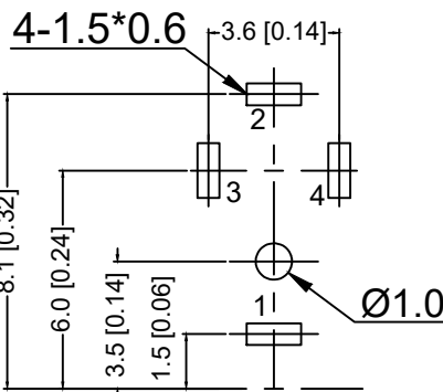
PCB HOLES(TOP VIEW) GENERAL TOLERANCE:0.1MM
