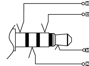
Matching Plug
