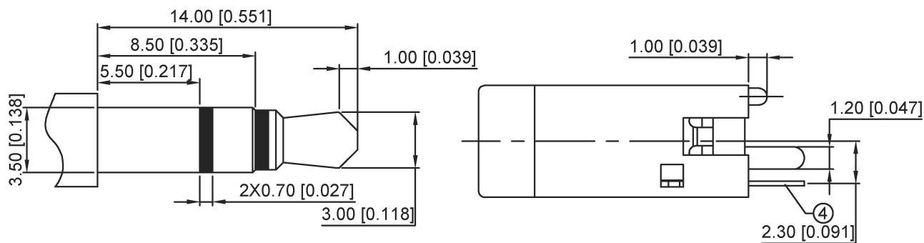
Ø3.50mm 3 POLE PLUG
