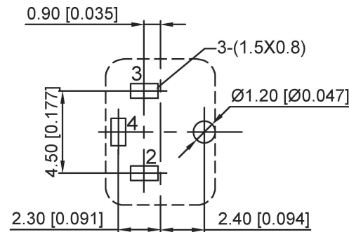
P.C.B LAYOUT MOUNTING PATTERN (TOP VIEW)
