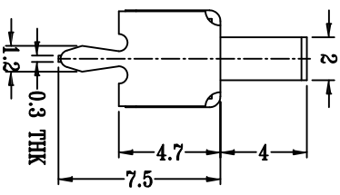
SCHMATIC (NON-SHORTING)
