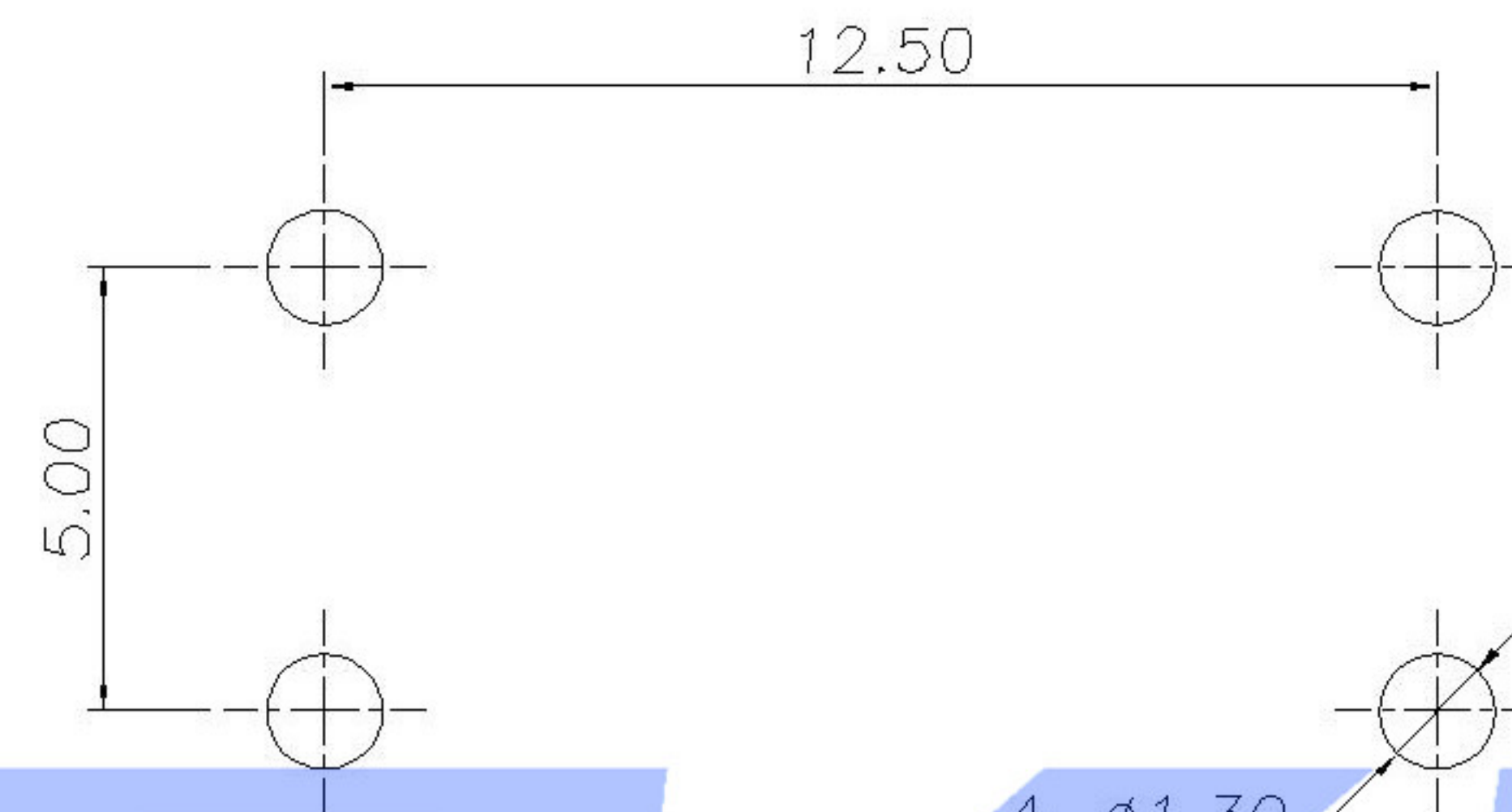
P.C.B Mounting pattern Dimension
