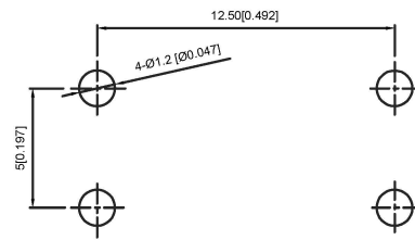
P.C.B MOUNTING PATTERN DIMENSION
