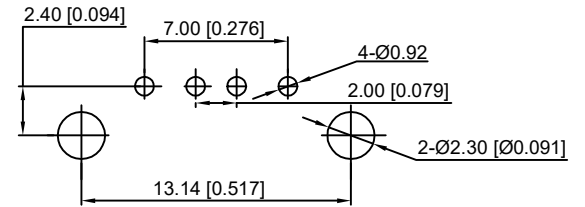
P.C.B LAYOUT BOTTOM VIEW
