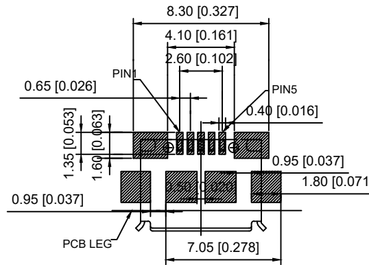
RECOMMENDED P.C.B. LAYOUT TOP VIEW (TOLRANCE: ±0.05)
