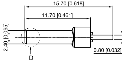
SECT B-B
