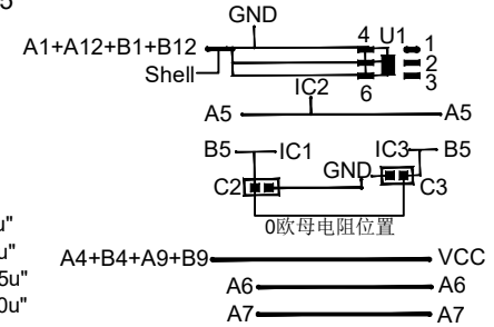
C TYPE PLUG:
