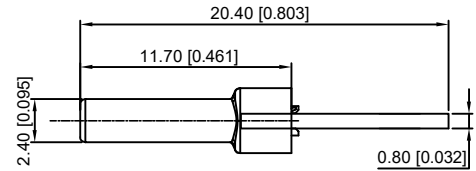
SECT B-B
