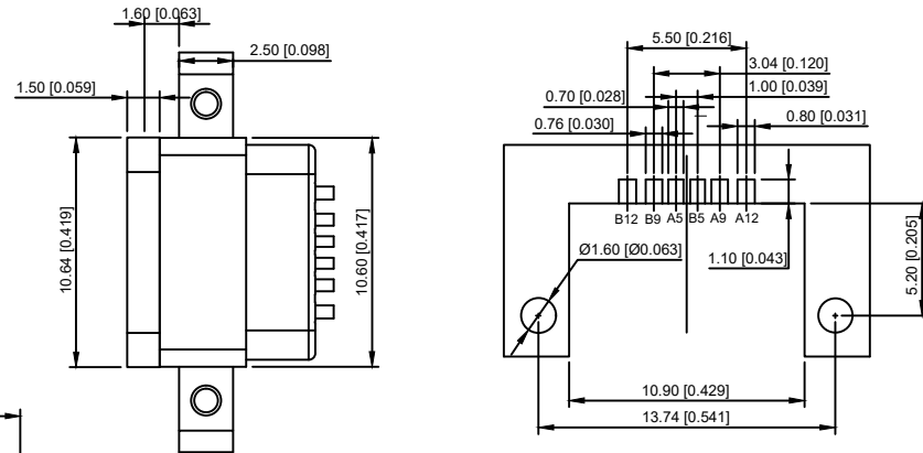
RECOMMENDED P.C.B LAYOUT TOLERANCE UNSPECIFIED ±0.05mm
