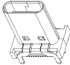
WITHOUT COVER
