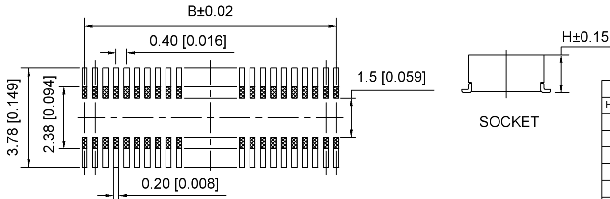
Recommended PCB Layout ±0.05
