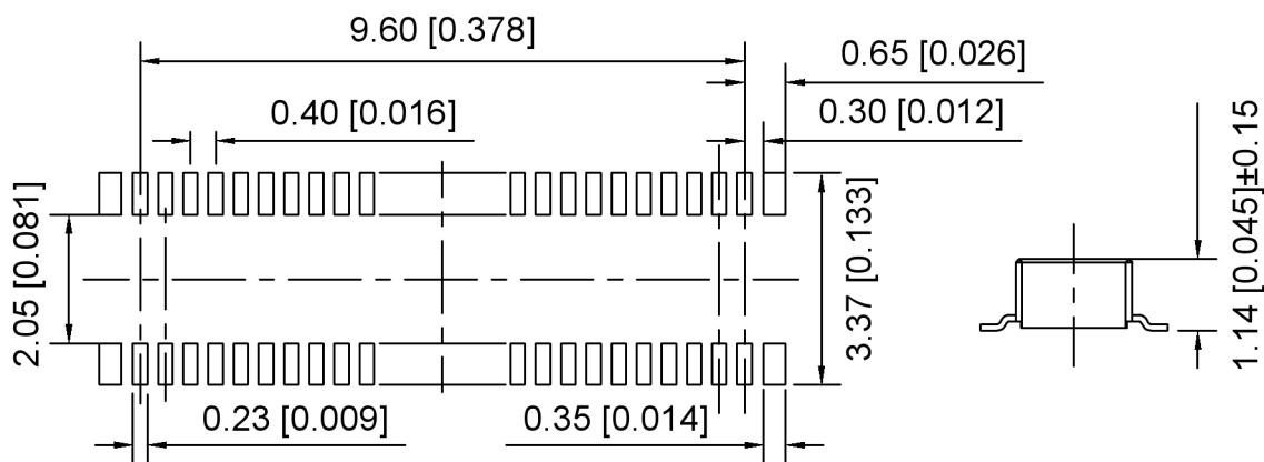
Recommended PCB Layout ±0.05
