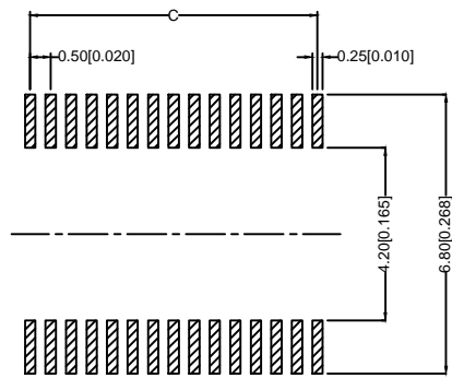
RECOMMENDED PCB PATTERN DIM. TOLERANCE : ±0.05
