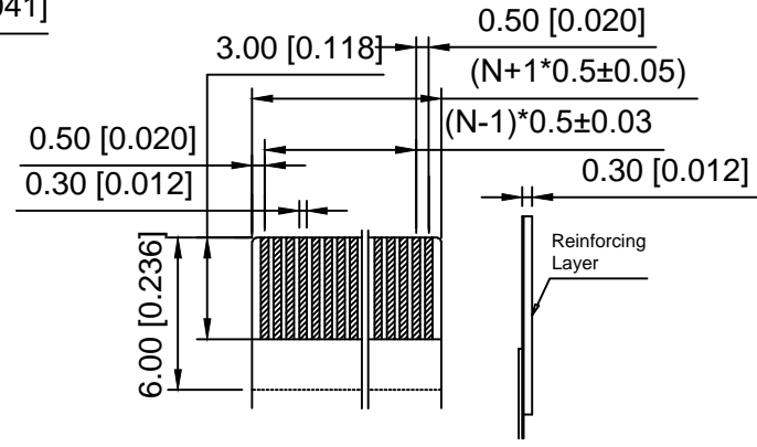
RECOMMENDED FFC/FPC DIM.
