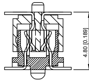
ASSEMBLY SCALE 2:1
