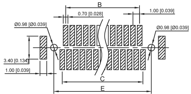
ASSEMBLY SCALE 2:1
