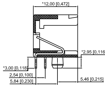
CUTAWAY VIEW
