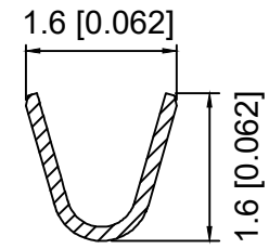
SECTION:A-A SCALE:1:1
