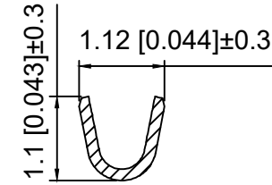
SECTION:B-B SCALE:1:1
