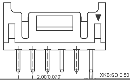
05P~13P Shape(Scale1:1) XKB:SQ 0.50
