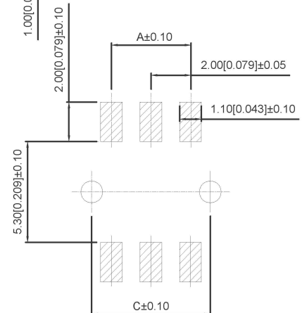
PCB LAYOUT
