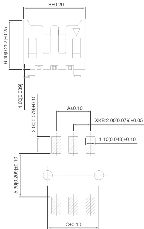
PCB LAYOUT
