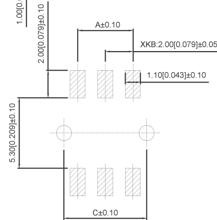
PCB LAYOUT
