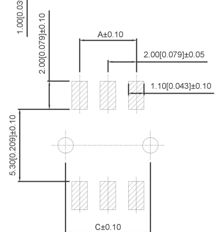
PCB LAYOUT
