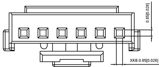
04P~20P Shape Scale 1:1
