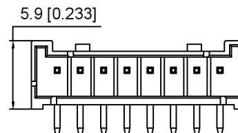
04~20P Shape (C1) Scale 1:1
