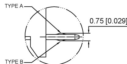
DETAIL A SCALE 2:1
