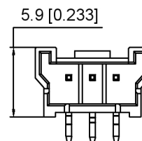
X3535WR-XXC1 Without Kink, With Stand off
