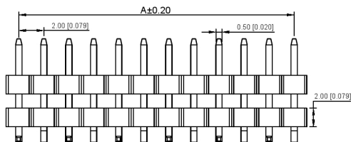
XJB Connectivity PCB LAYOUT
