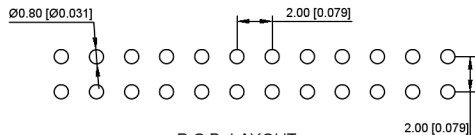
P.C.B LAYOUT XXB Connectivity
