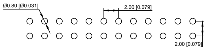
P.C.B LAYOUT XKB Connectivity
