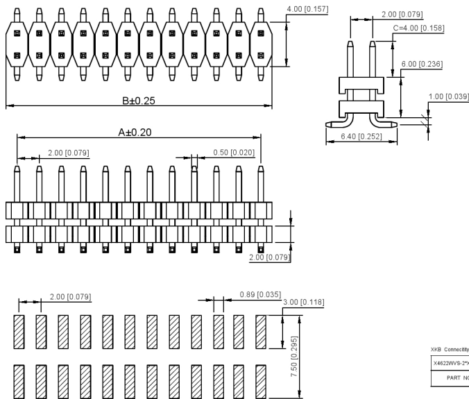
XKB Connectivity P.C.B LAYOUT
