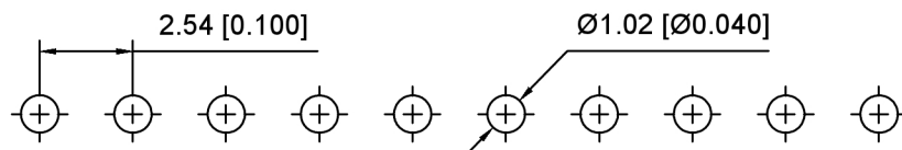
PCB LAYOUT
