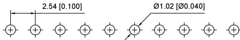
PCB LAYOUT
