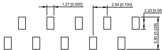
PCB LAYOUT R1 TYPE
