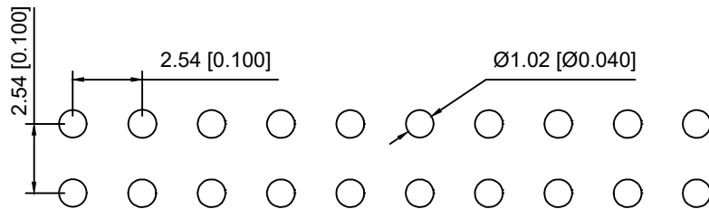
PCB LAYOUT
