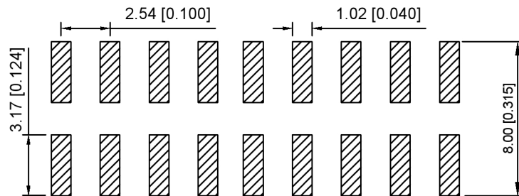
PCB LAYOUT
