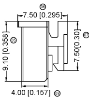
3P~15P Shape
