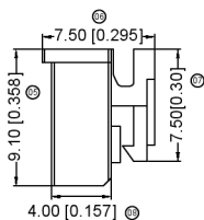
3P~15P Shape
