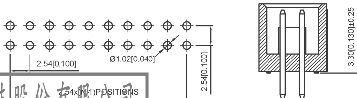
Recommended PCB Layout PCB Board Tolerance±0.05
