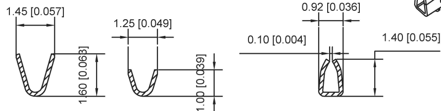
SECTION:C-C SCALE:1:1
