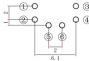
PCB LAYOT
