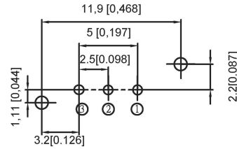
P.C.B LAYOUT MOUNTING PATTERN
