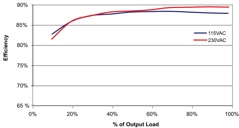
Figure 9 - ECS65US24
