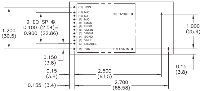
BOTTOM VIEW
