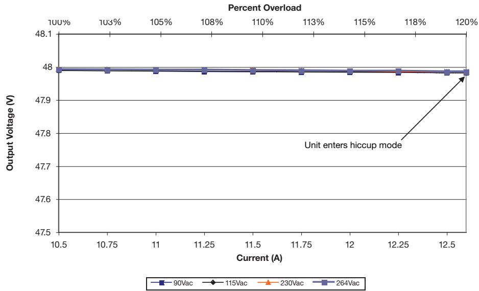
Figure 3 - LCL500PS48
