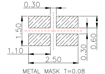
TOLERANCE:±0.05MM (FOR REFERENCE ONLY)
