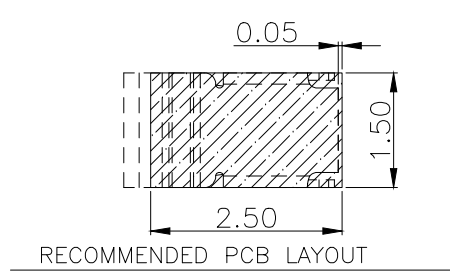
TOLERANCE:±0.05MM (FOR REFERENCE ONLY)
