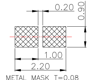
METAL MASK T=0.08
