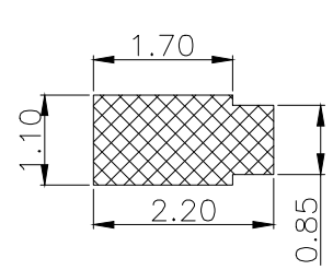
RECOMMENDED PCB LAYOUT TOLERANCE: ±0.05MM (FOR REFERENCE ONLY)
